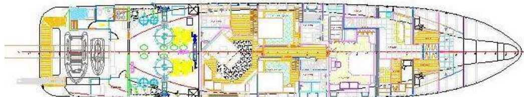
LOWER DECK 12.00m x 3.00m
